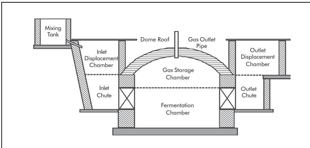
Figure 2.9: Fixed Dome Biogas Plant
